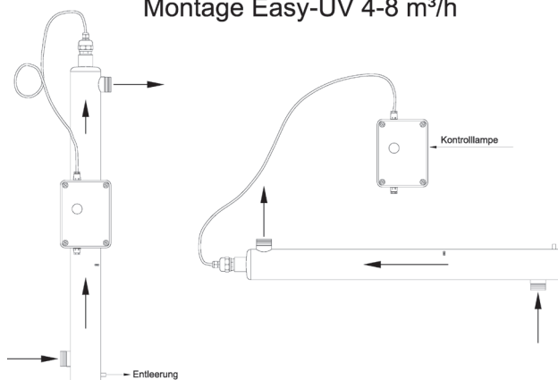
Montage Easy-UV 4-8 m 3 /h
